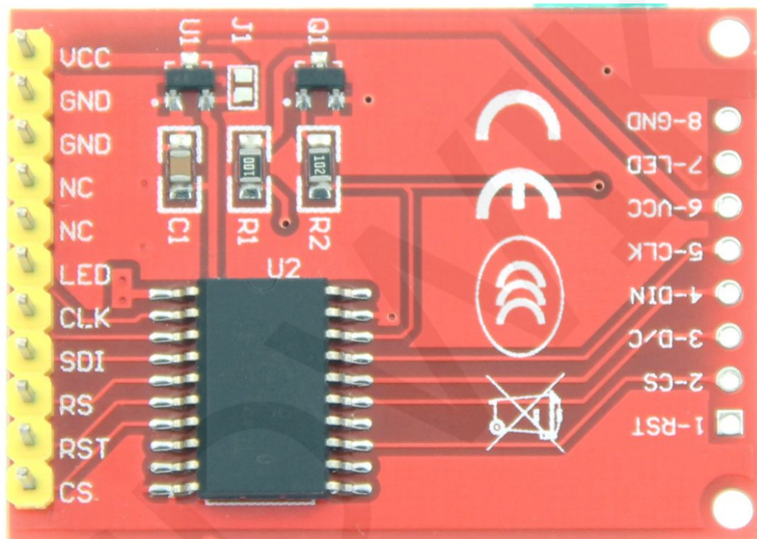
Picture1. Pin silkscreen picture
